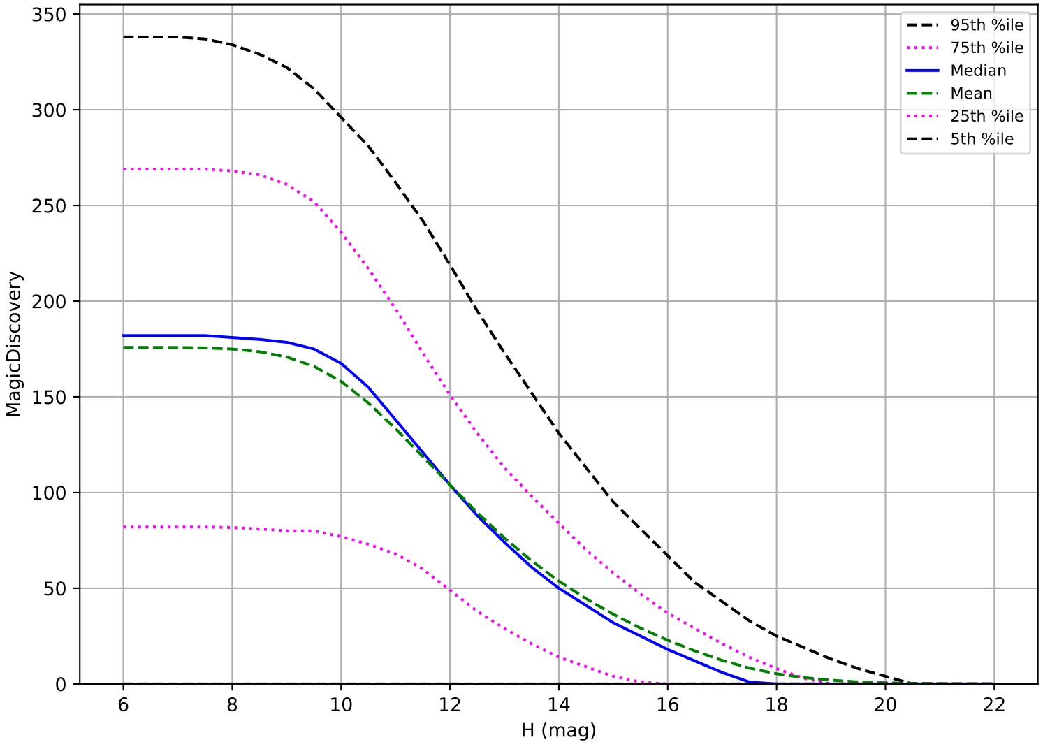
internal_u_expt45_nscale1.0v3.4_10yrs: OCC_r5 6 detections in 60 nights detection loss
