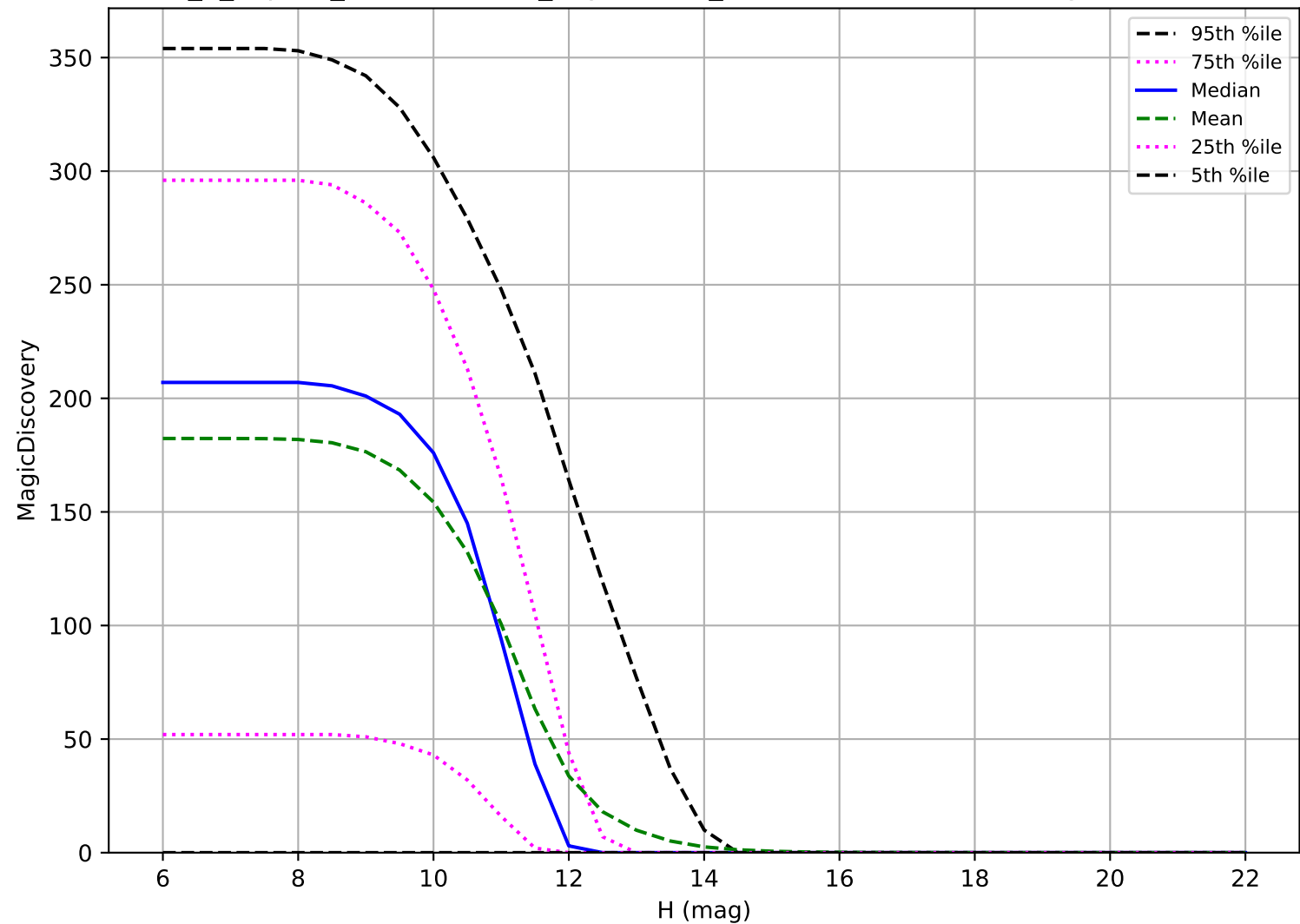
internal_u_expt45_nscale1.0v3.4_10yrs: OCC_r20 6 detections in 60 nights detection loss
