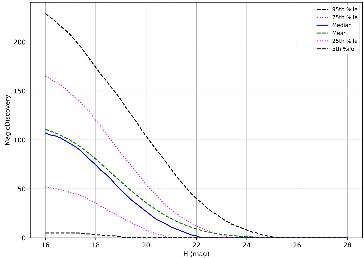
internal_u_expt45_nscale1.0v3.4_10yrs: NEO 6 detections in 60 nights detection loss
