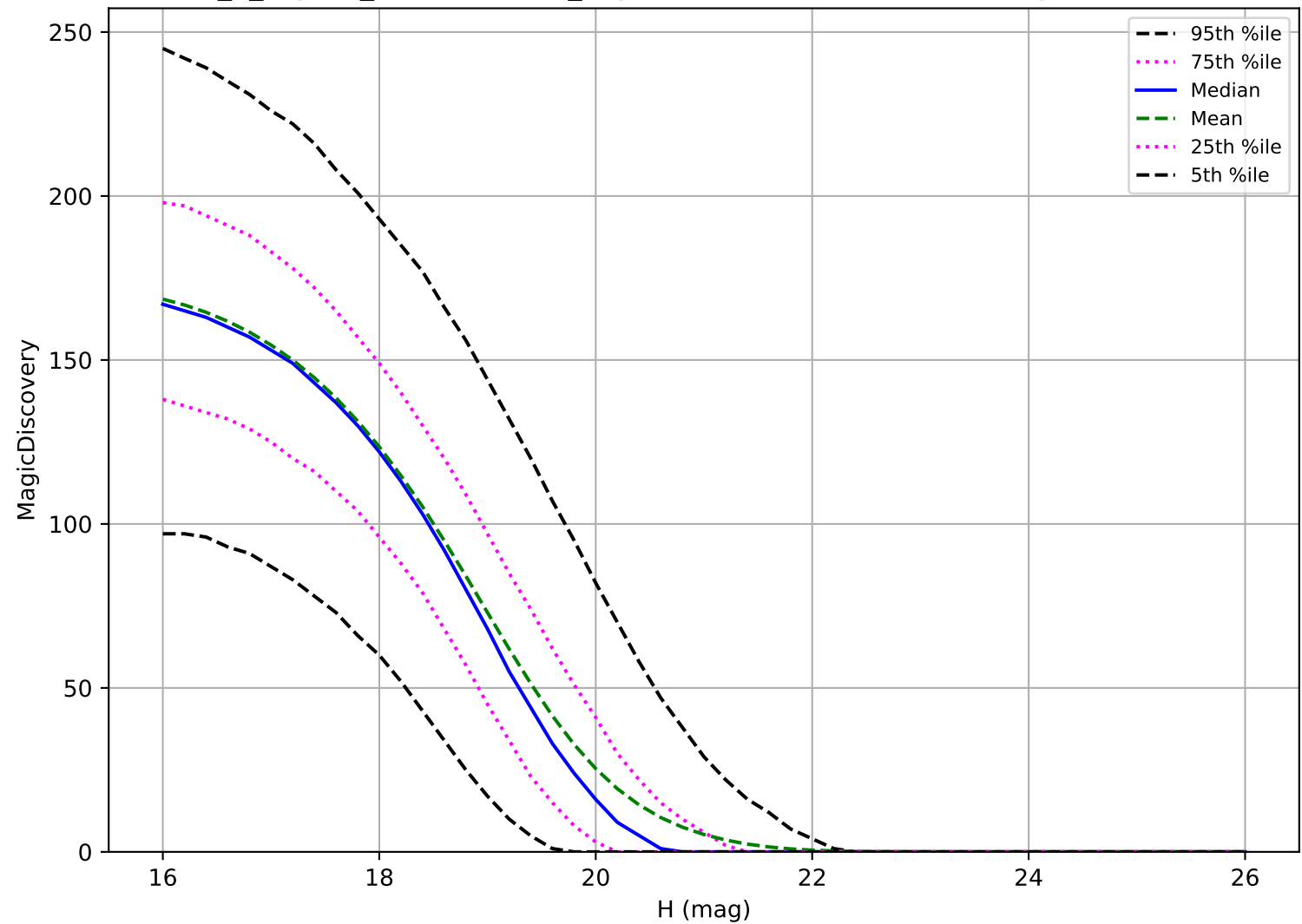
internal_u_expt45_nscale1.0v3.4_10yrs: MBA 6 detections in 60 nights detection loss
