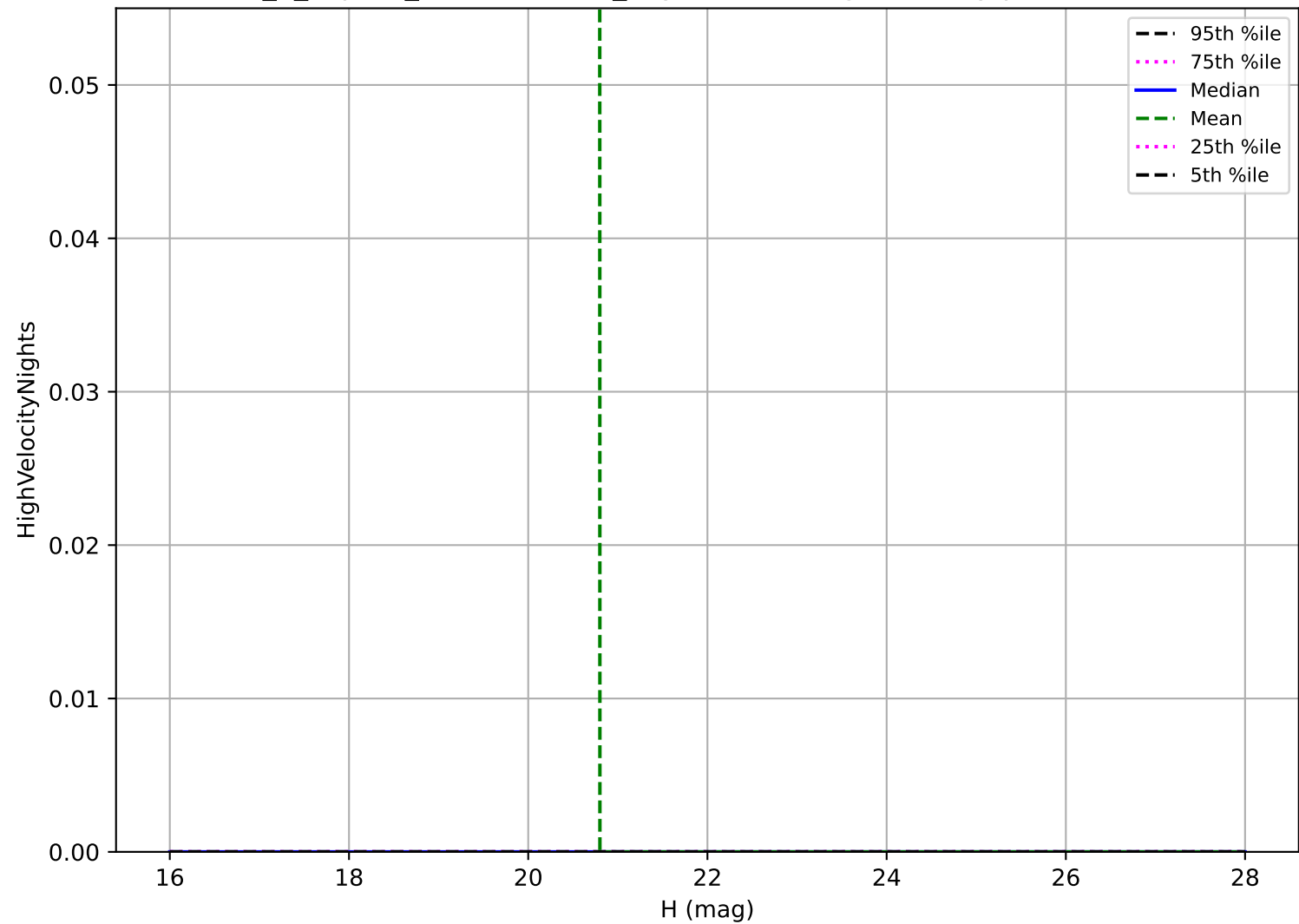
internal_u_expt45_nscale1.0v3.4_10yrs: Vatira High velocity pair detection loss
