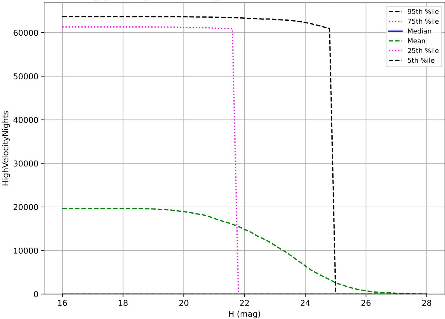
internal_u_expt45_nscale1.0v3.4_10yrs: NEO High velocity pair detection loss
