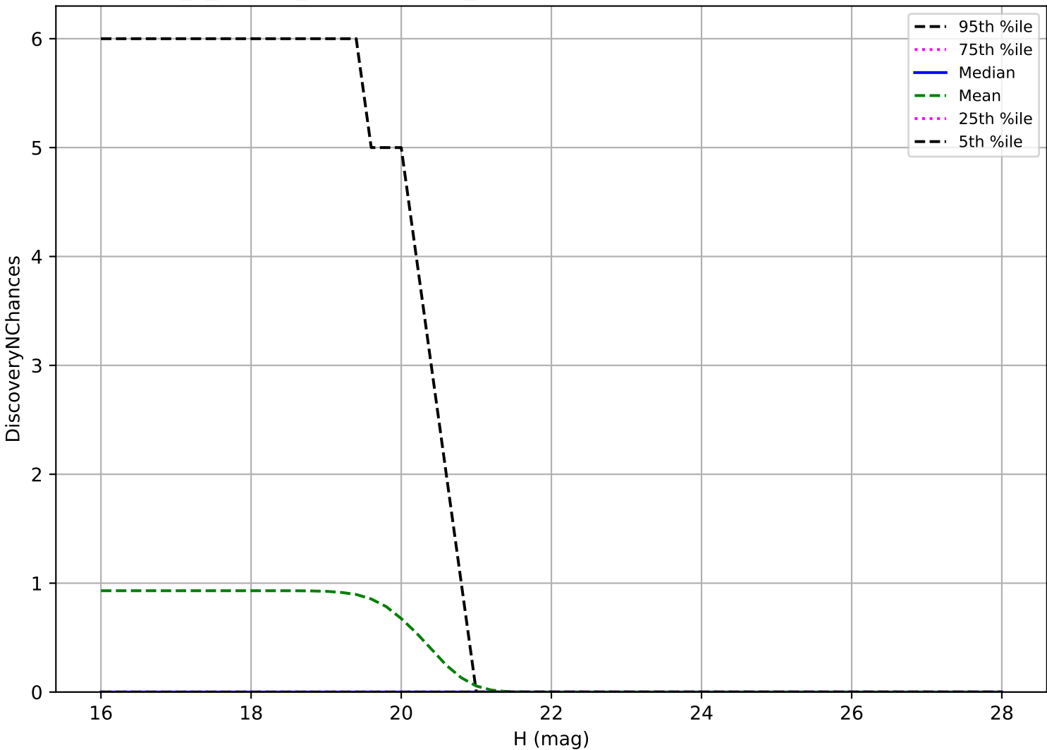
internal_u_expt45_nscale1.0v3.4_10yrs: Vatira 3 pairs in 15 nights detection loss
