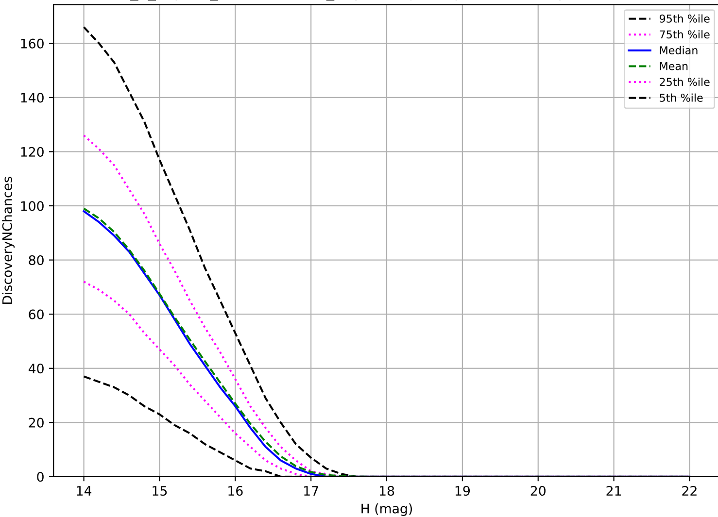
internal_u_expt45_nscale1.0v3.4_10yrs: Trojan 3 pairs in 15 nights detection loss
