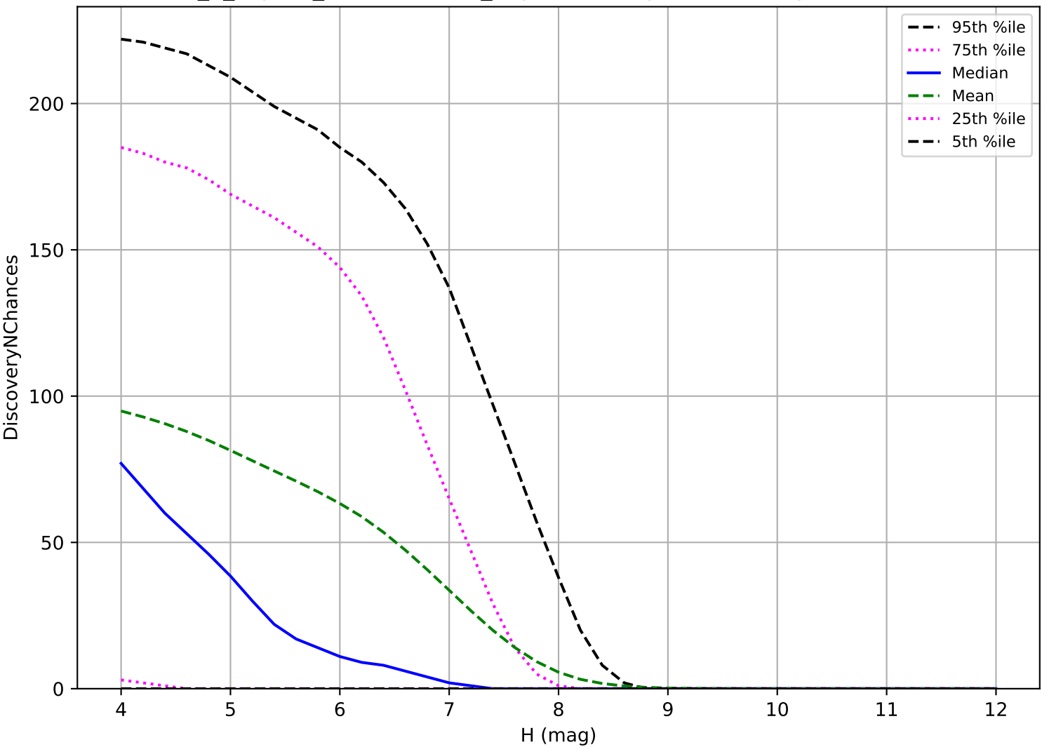
internal_u_expt45_nscale1.0v3.4_10yrs: TNO 3 pairs in 15 nights detection loss
