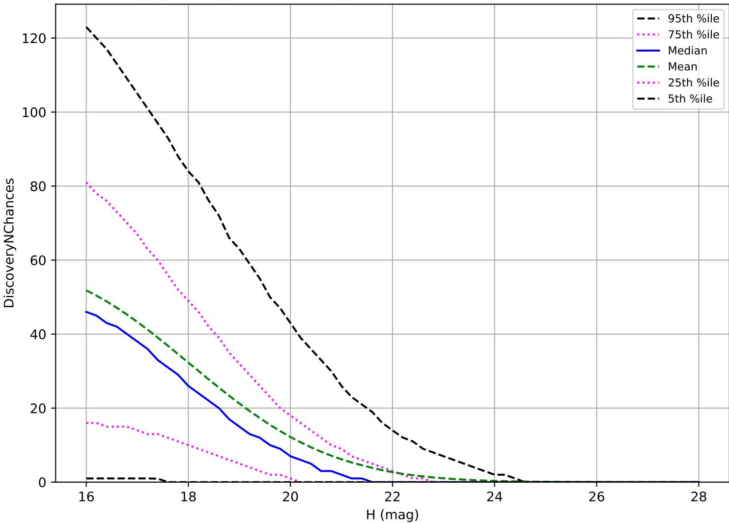
internal_u_expt45_nscale1.0v3.4_10yrs: PHA 3 pairs in 15 nights detection loss
