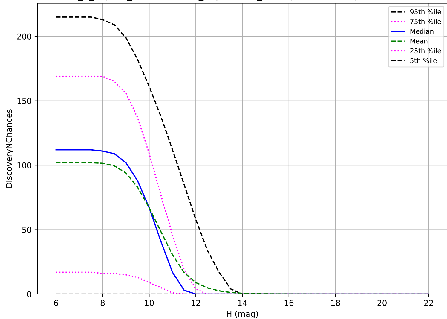
internal_u_expt45_nscale1.0v3.4_10yrs: OCC_r20 3 pairs in 15 nights detection loss
