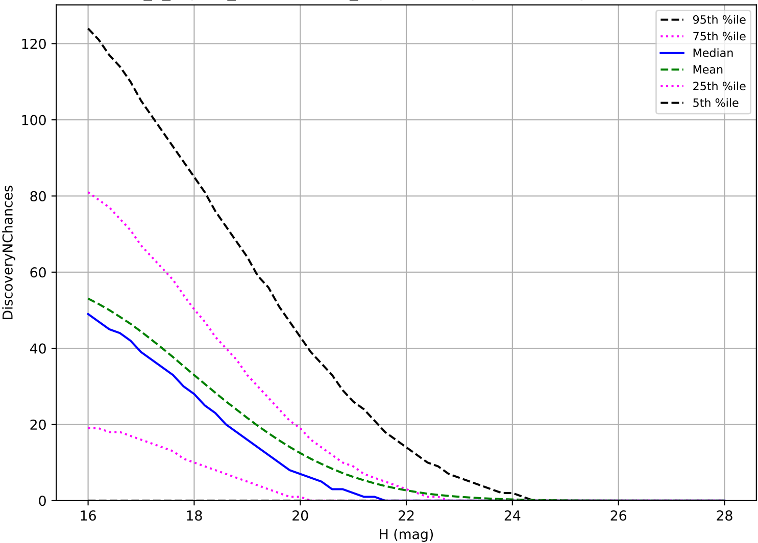
internal_u_expt45_nscale1.0v3.4_10yrs: NEO 3 pairs in 15 nights detection loss
