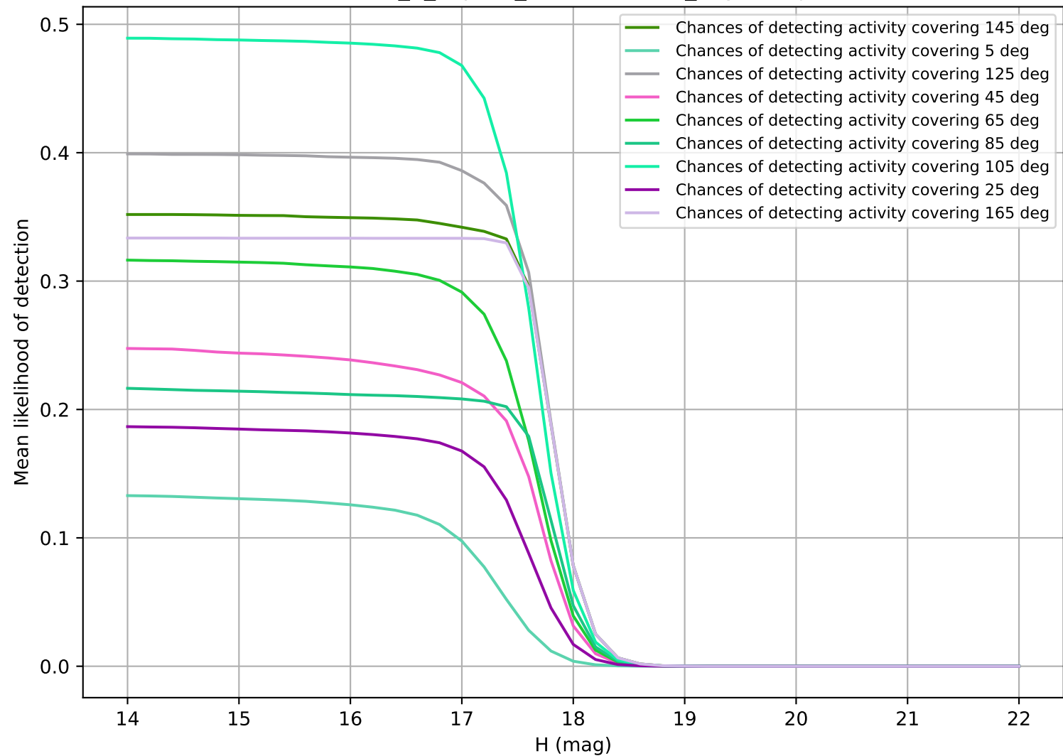
internal_u_expt45_nscale1.0v3.4_10yrs Trojan
