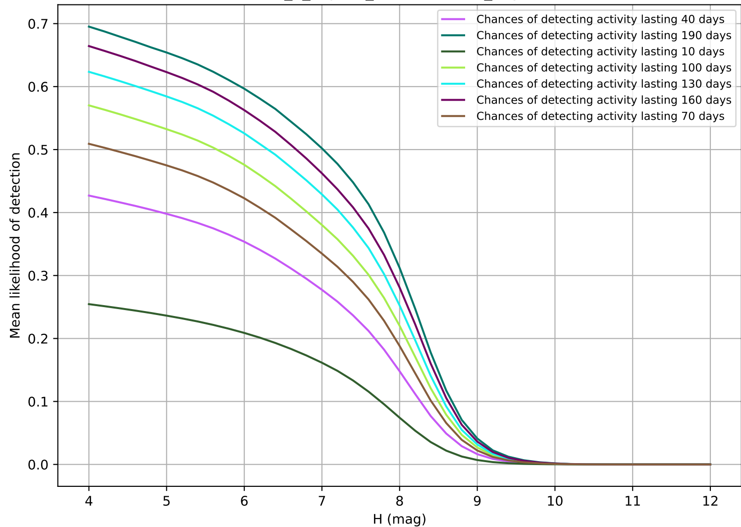
internal_u_expt45_nscale1.0v3.4_10yrs TNO
