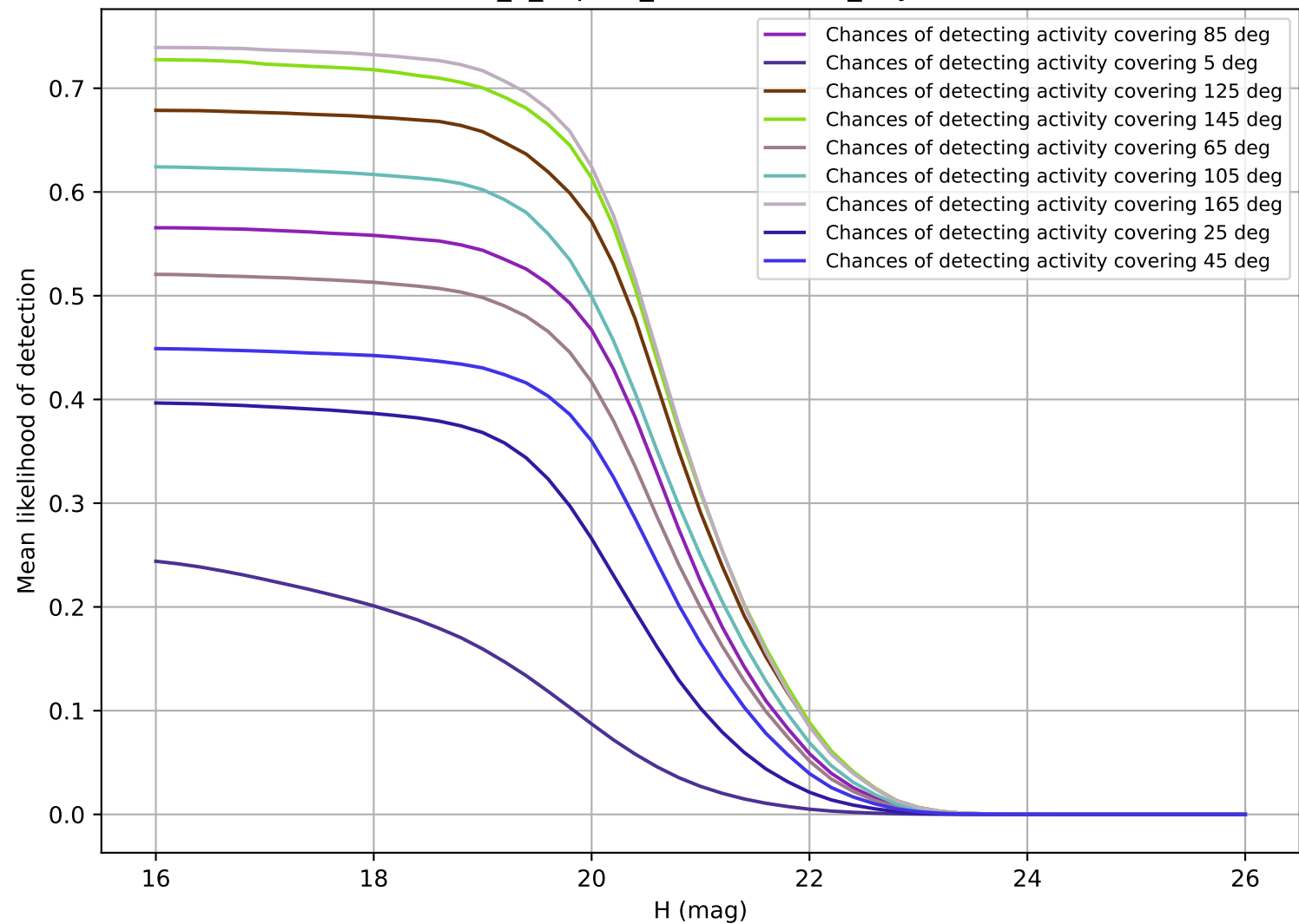
internal_u_expt45_nscale1.0v3.4_10yrs MBA
