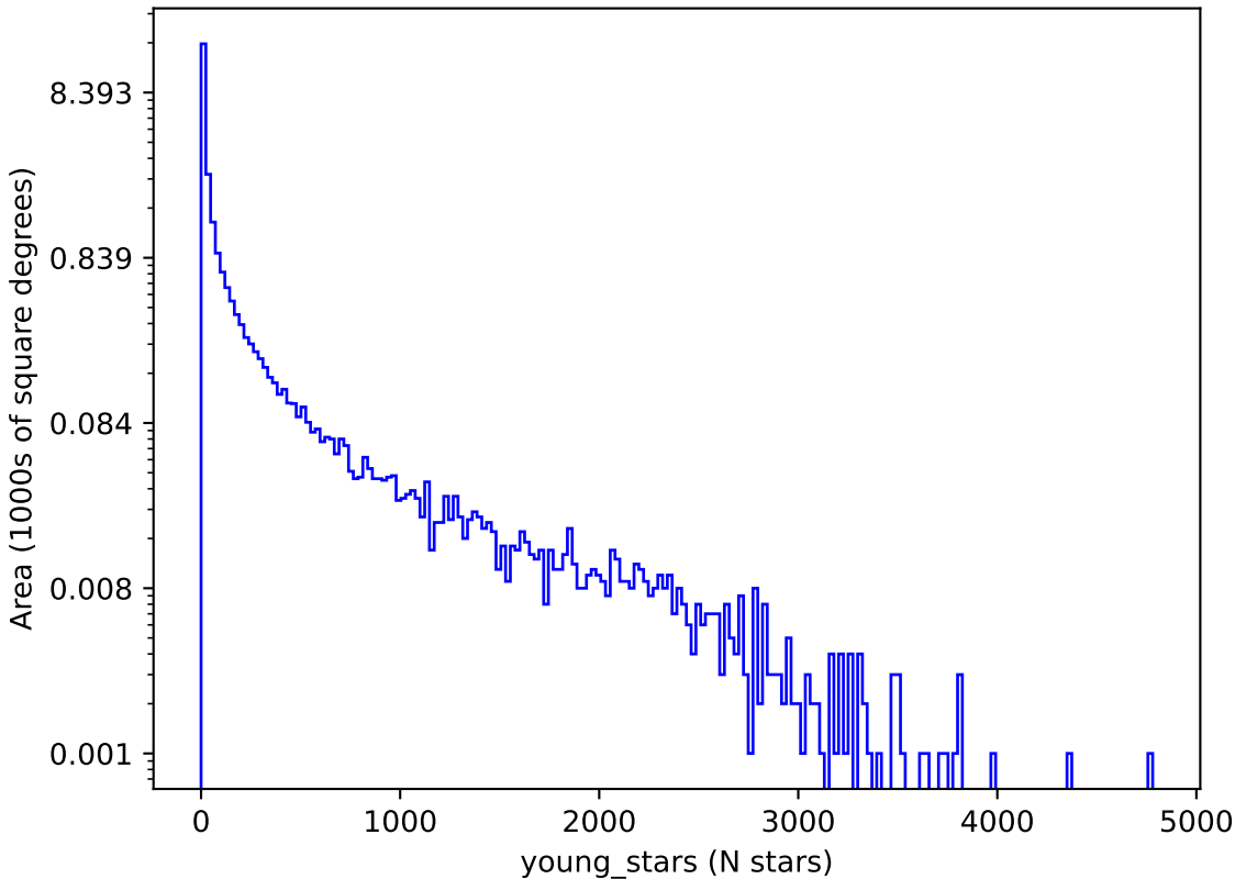
internal_u_expt45_nscale1.0v3.4_10yrs : young_stars
