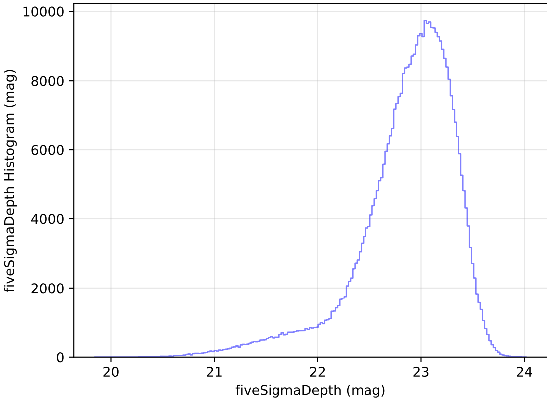
internal_u_expt45_nscale1.0v3.4_10yrs z: fiveSigmaDepth Histogram
