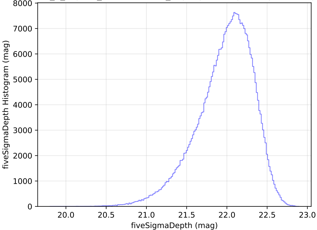
internal_u_expt45_nscale1.0v3.4_10yrs y: fiveSigmaDepth Histogram
