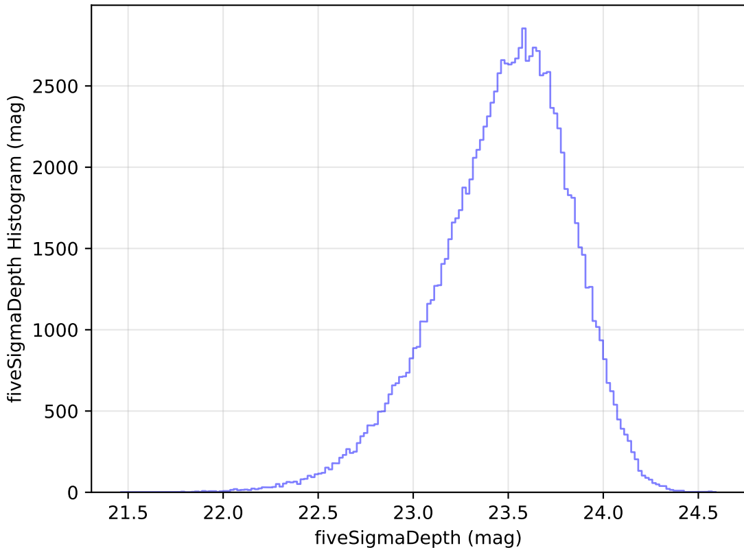
internal_u_expt45_nscale1.0v3.4_10yrs u: fiveSigmaDepth Histogram
