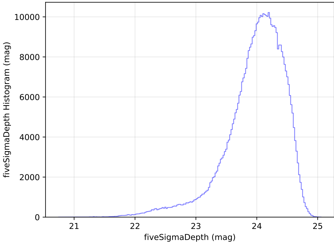
internal_u_expt45_nscale1.0v3.4_10yrs r: fiveSigmaDepth Histogram
