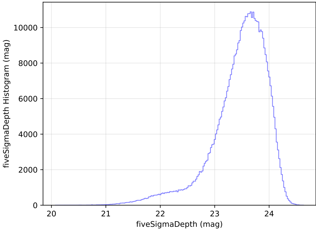
internal_u_expt45_nscale1.0v3.4_10yrs i: fiveSigmaDepth Histogram
