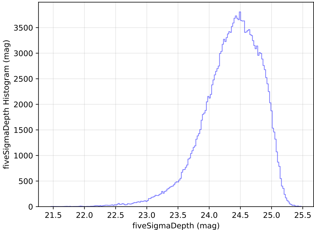
internal_u_expt45_nscale1.0v3.4_10yrs g: fiveSigmaDepth Histogram
