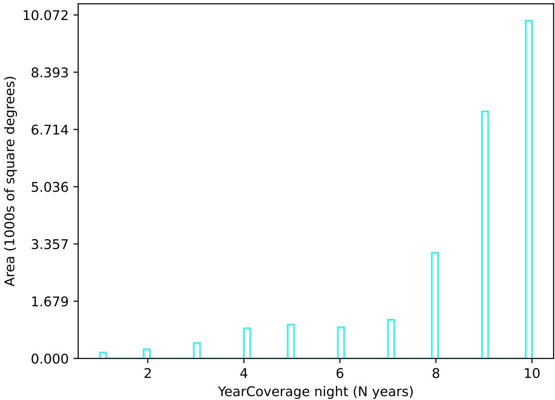
internal_u_expt45_nscale1.0v3.4_10yrs u band: YearCoverage night
