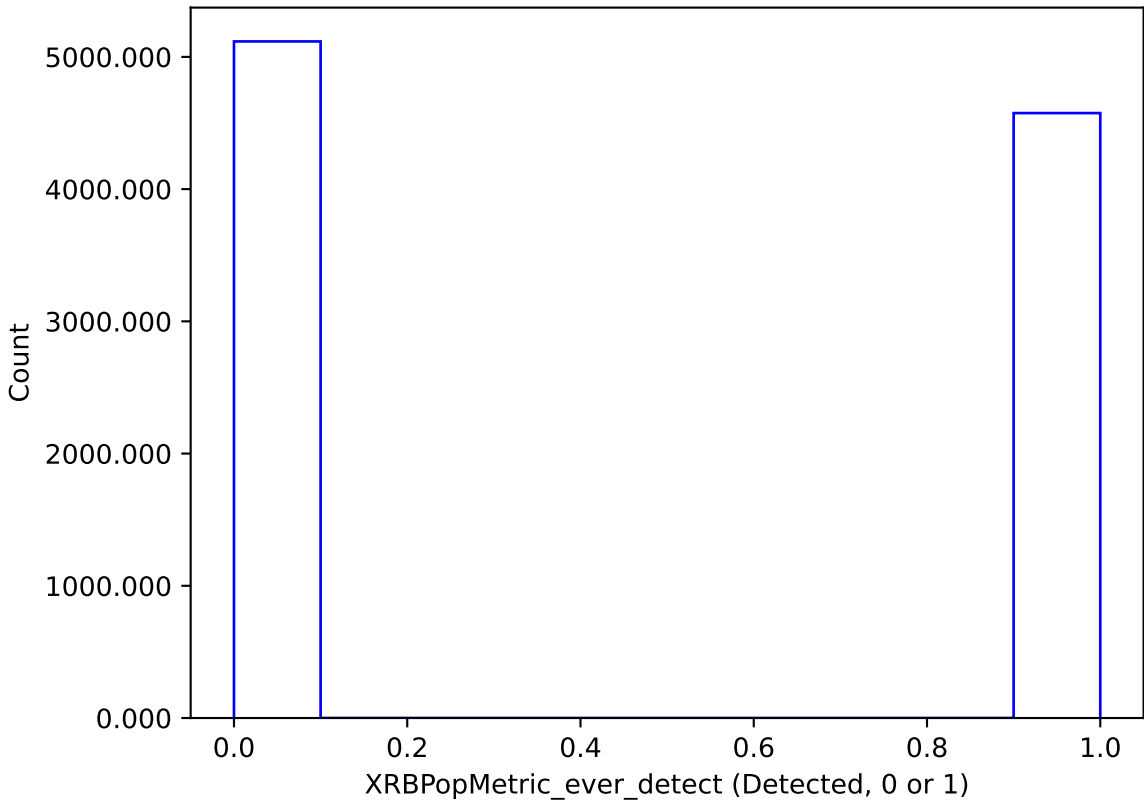
internal_u_expt45_nscale1.0v3.4_10yrs : XRBPoMetric_ever_detect
