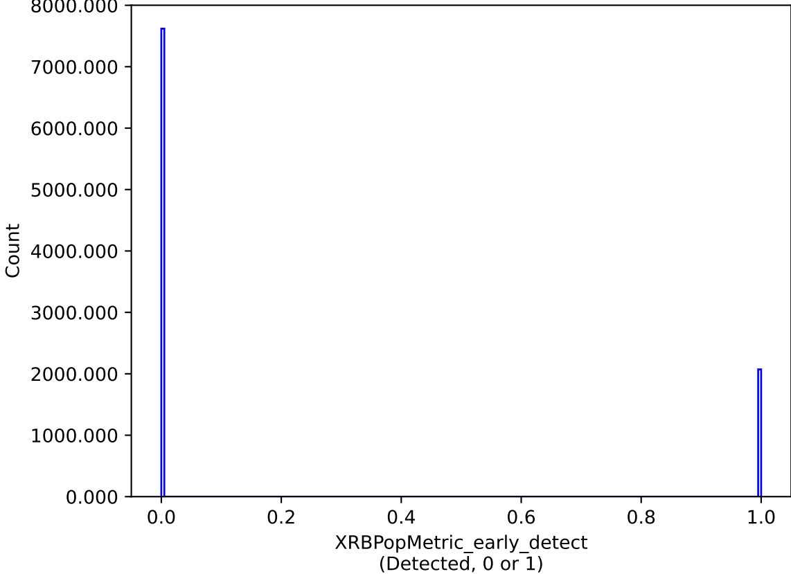
internal_u_expt45_nscale1.0v3.4_10yrs : XRBPoMetric_early_detect
