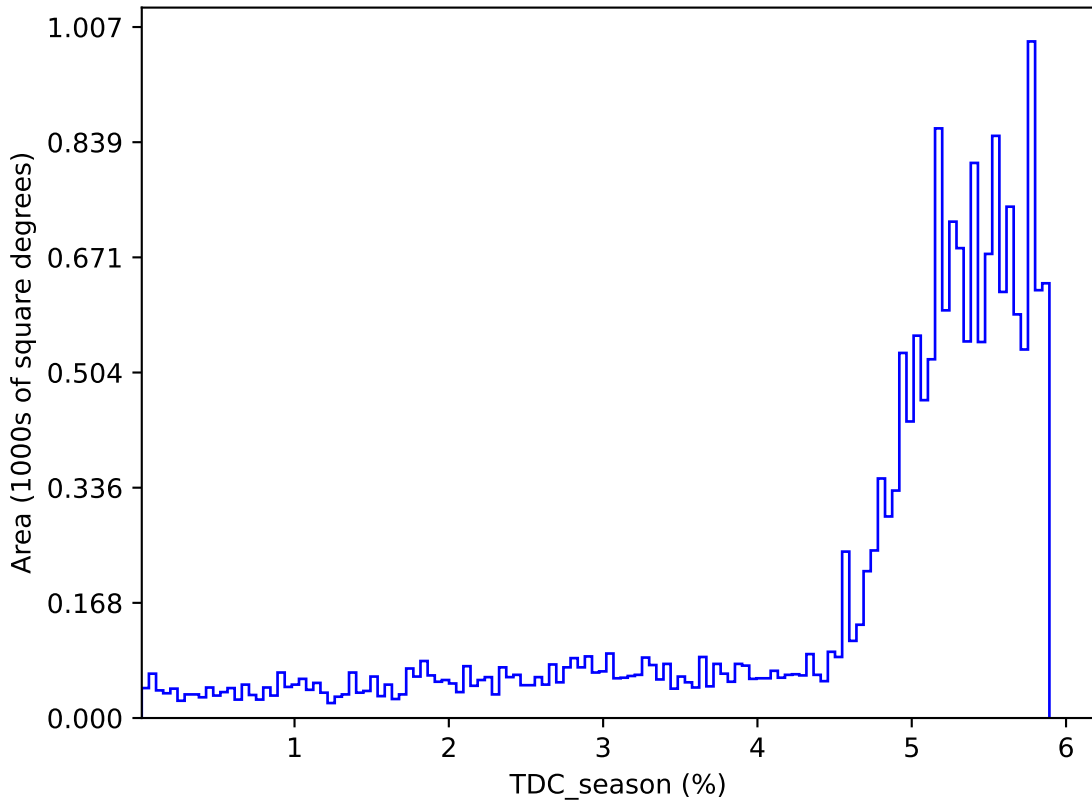
internal_u_expt45_nscale1.0v3.4_10yrs : TDC_season
