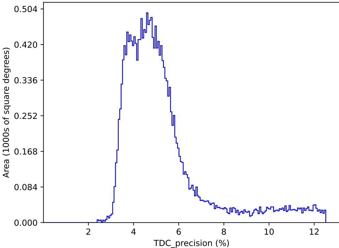
internal_u_expt45_nscale1.0v3.4_10yrs : TDC_precision
