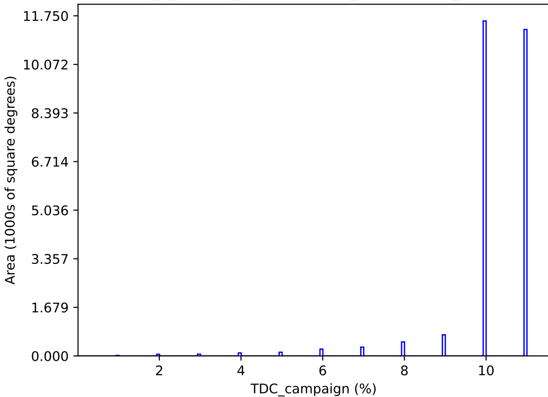
internal_u_expt45_nscale1.0v3.4_10yrs : TDC_campaign
