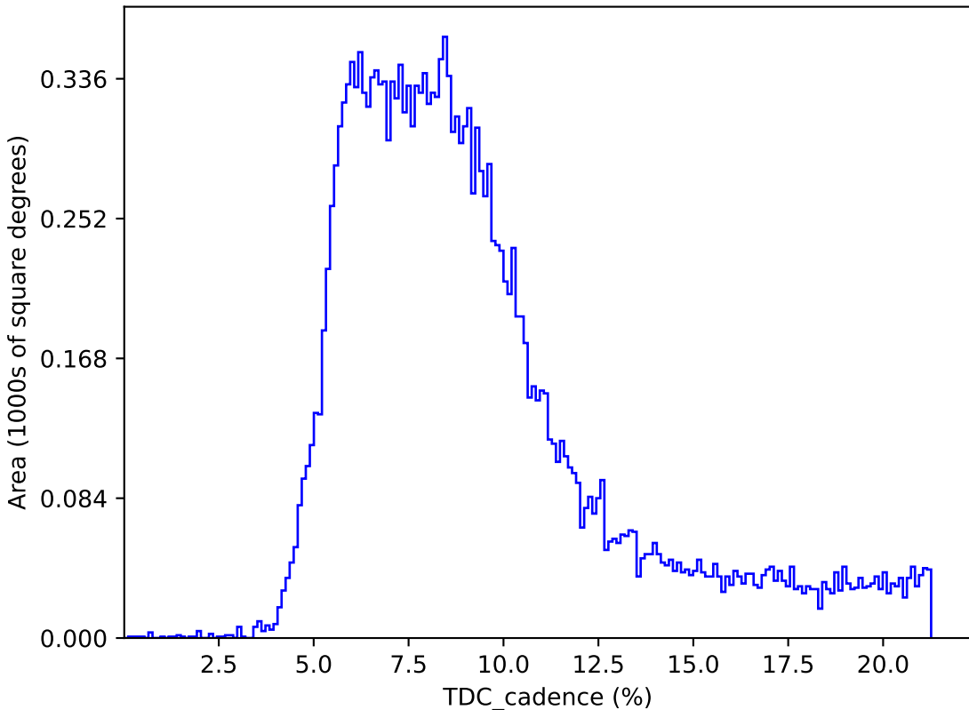
internal_u_expt45_nscale1.0v3.4_10yrs : TDC_cadence
