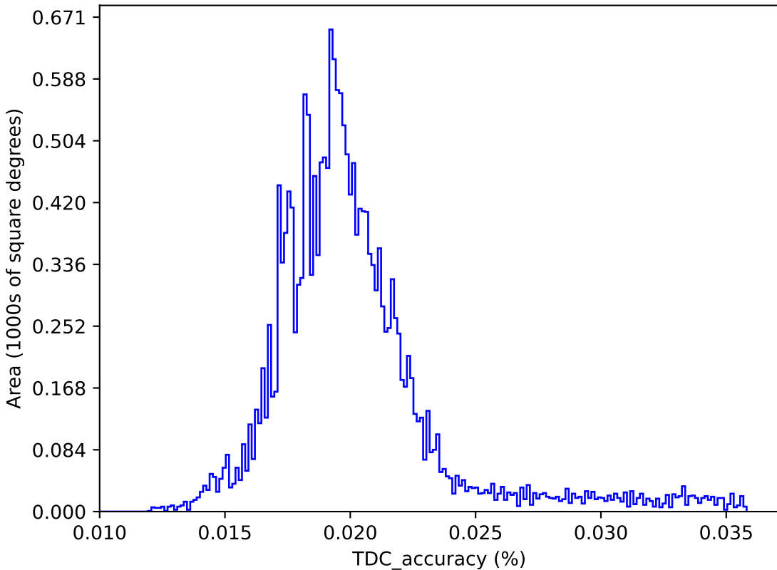
internal_u_expt45_nscale1.0v3.4_10yrs : TDC_accuracy
