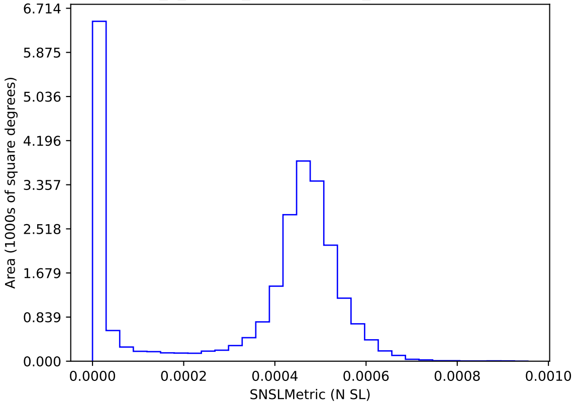
internal_u_expt45_nscale1.0v3.4_10yrs : SNSLMetric
