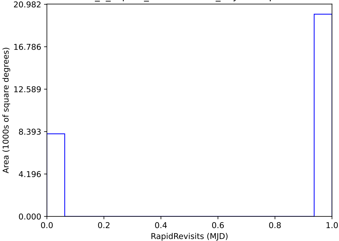
internal_u_expt45_nscale1.0v3.4_10yrs : RapidRevisits
