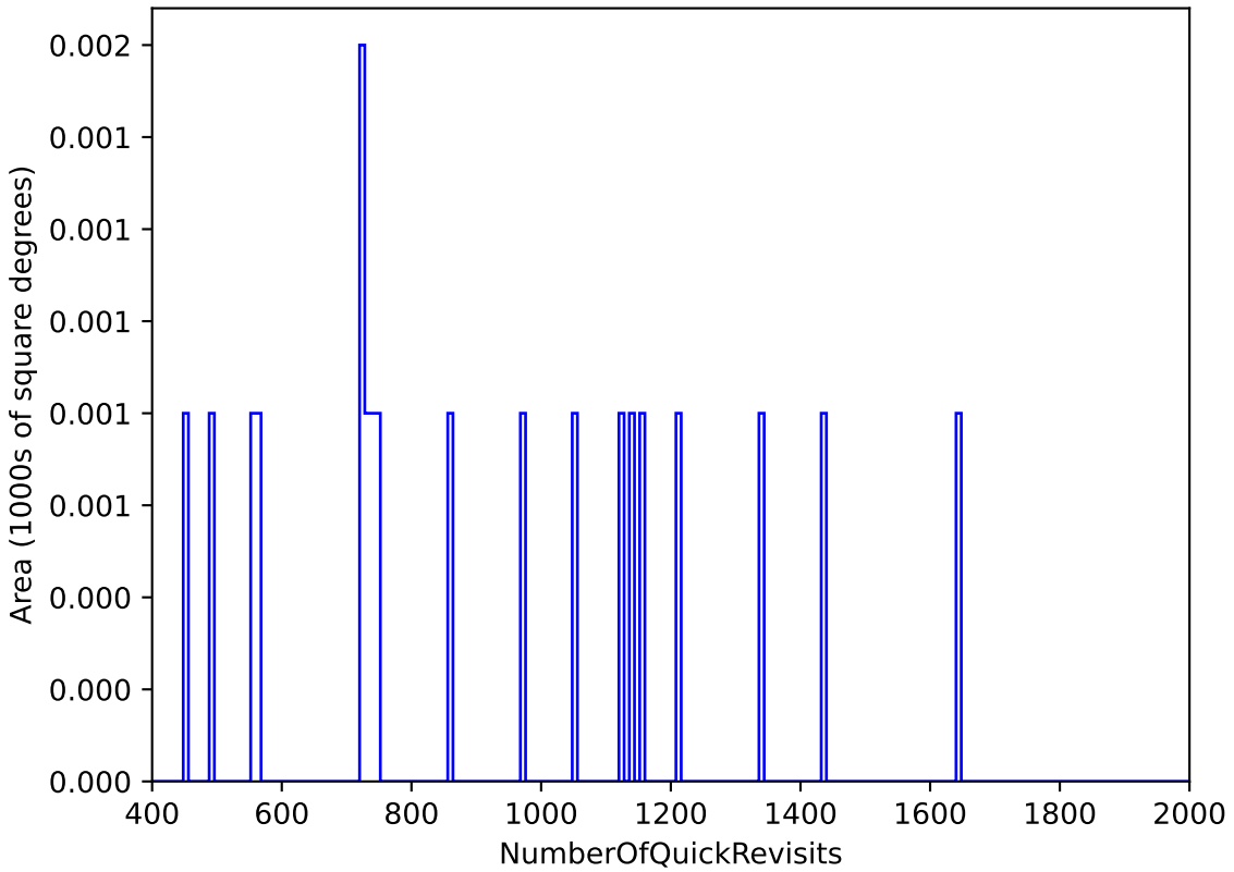
internal_u_expt45_nscale1.0v3.4_10yrs : NumberOfQuickRevisits
