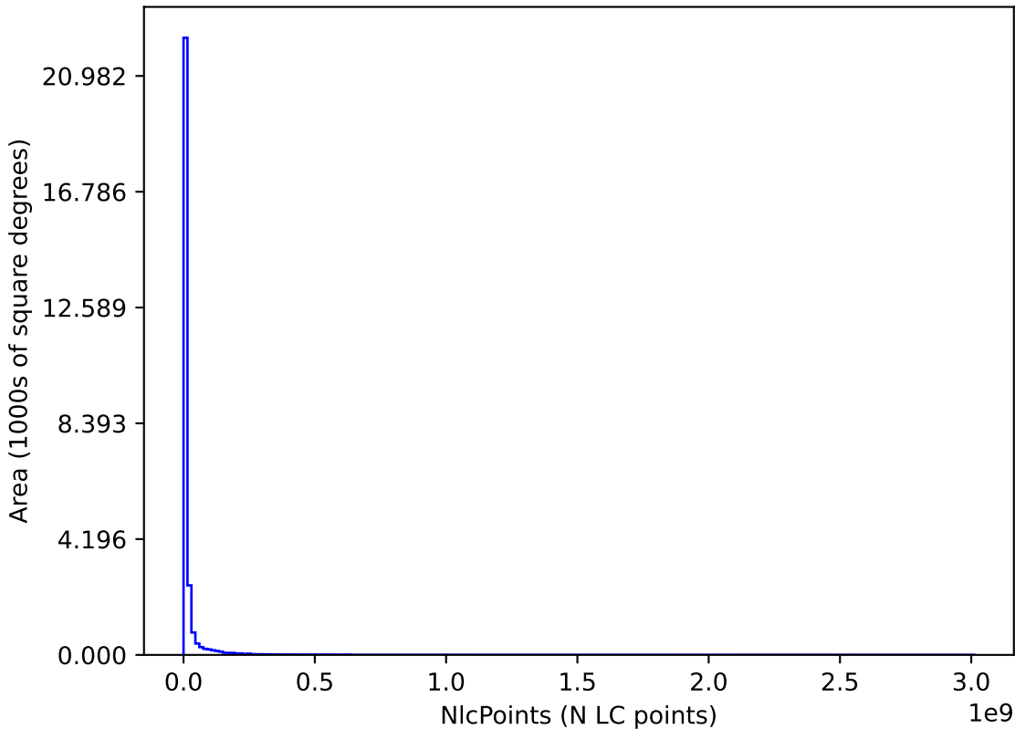
internal_u_expt45_nscale1.0v3.4_10yrs : NlcPoints
