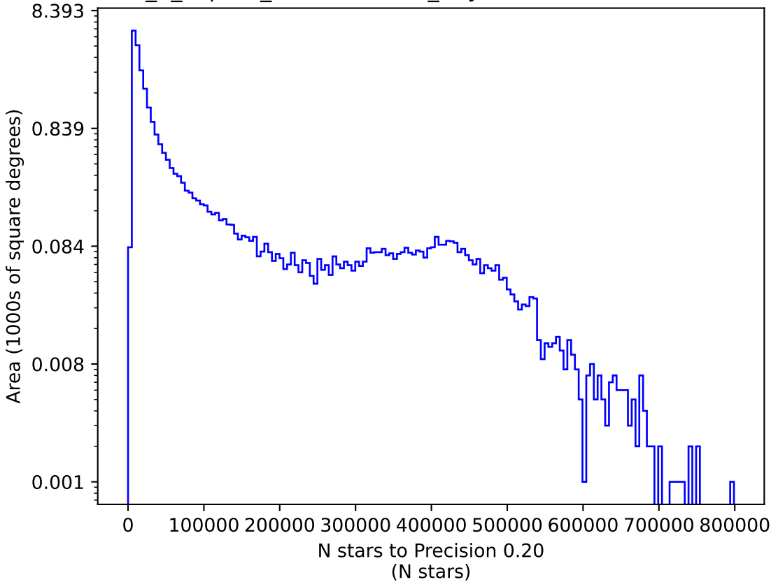
internal_u_expt45_nscale1.0v3.4_10yrs i: N stars to Precision 0.20
