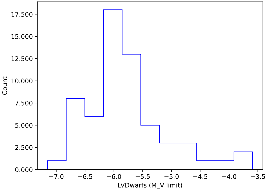
internal_u_expt45_nscale1.0v3.4_10yrs gi: LVDwarfs
