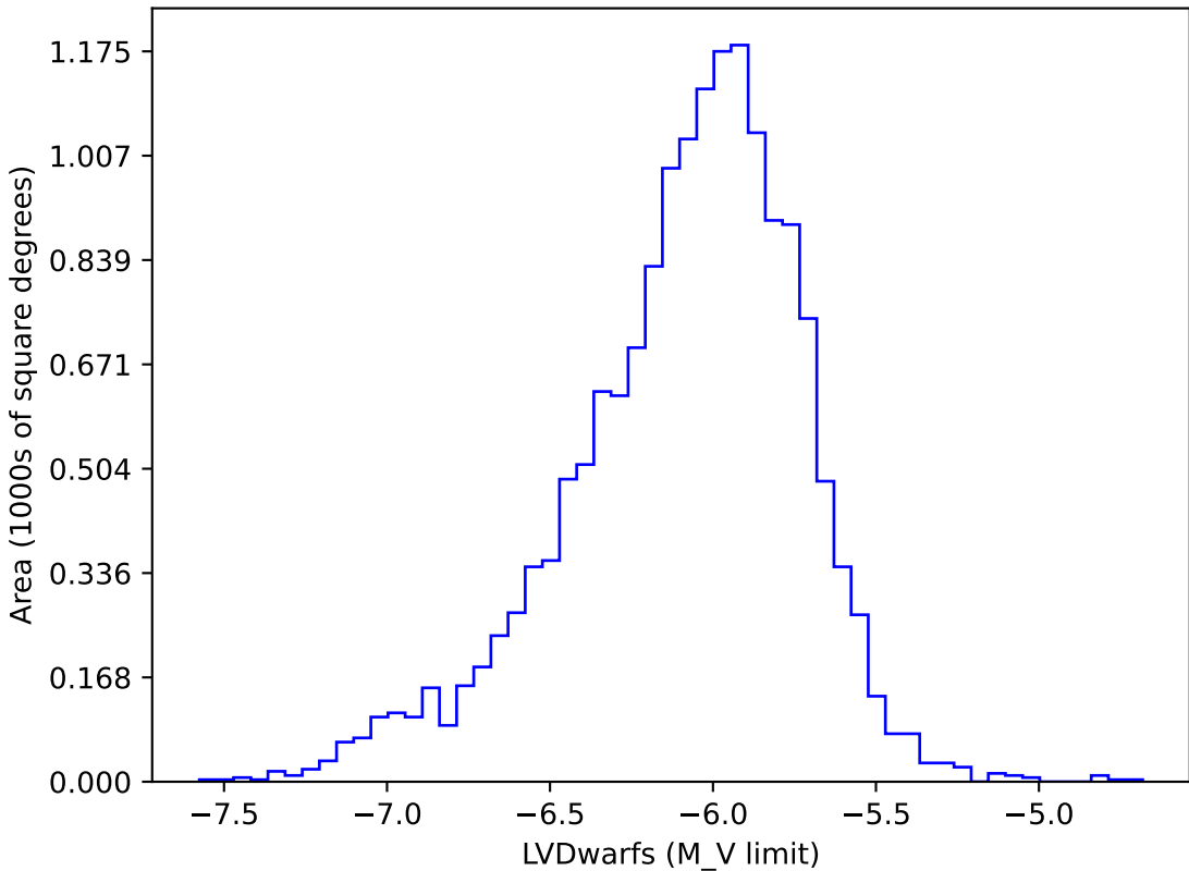
internal_u_expt45_nscale1.0v3.4_10yrs gi: LVDwarfs
