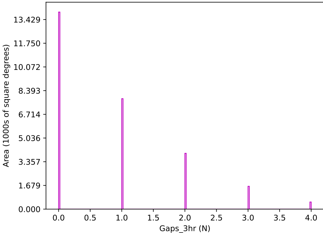
internal_u_expt45_nscale1.0v3.4_10yrs z band: Gaps_3hr
