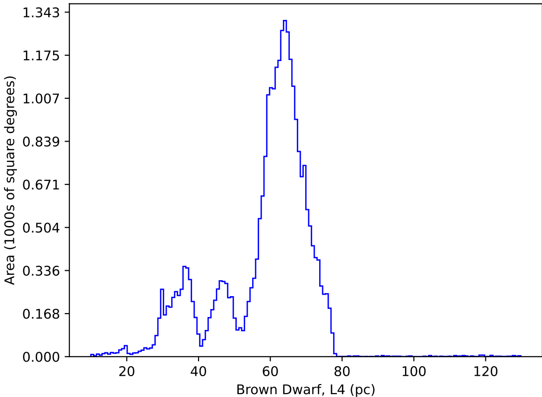
internal_u_expt45_nscale1.0v3.4_10yrs : Brown Dwarf, L4
