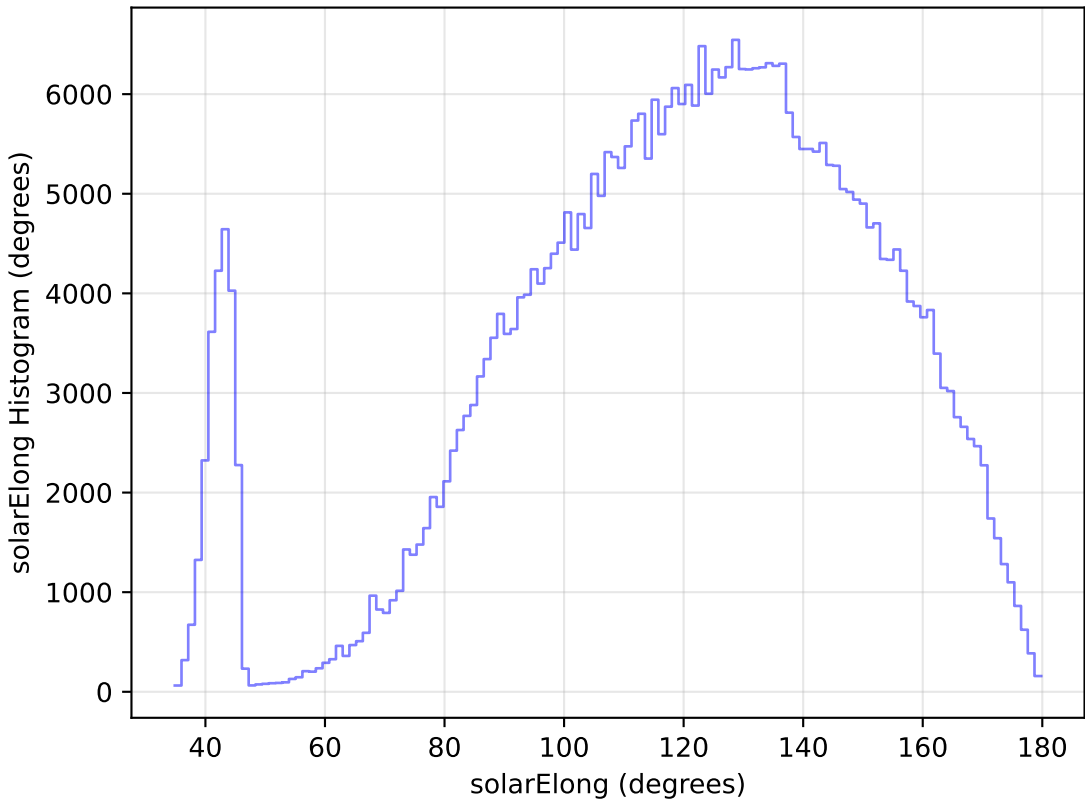
internal_u_expt45_nscale1.0v3.4_10yrs WFD z band: solarElong Histogram
