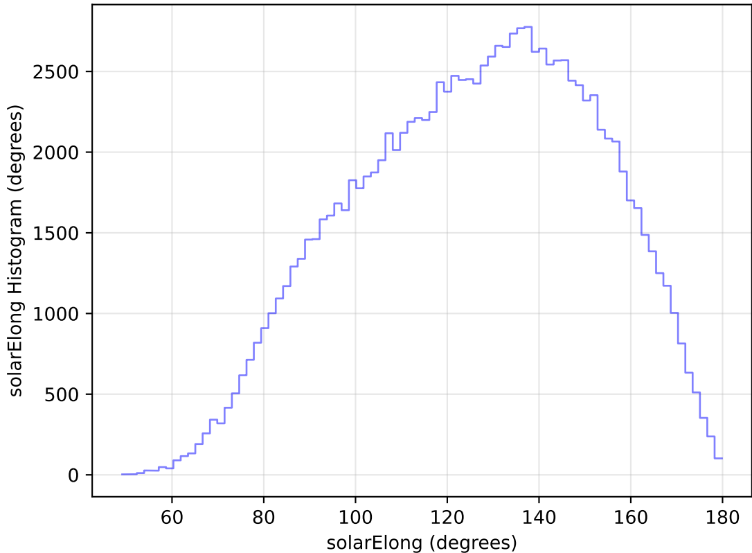
internal_u_expt45_nscale1.0v3.4_10yrs WFD u band: solarElong Histogram
