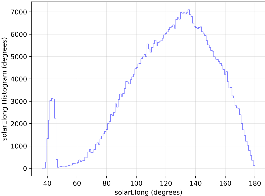
internal_u_expt45_nscale1.0v3.4_10yrs WFD r band: solarElong Histogram
