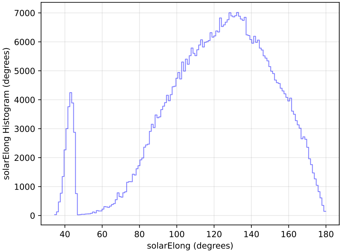
internal_u_expt45_nscale1.0v3.4_10yrs WFD i band: solarElong Histogram
