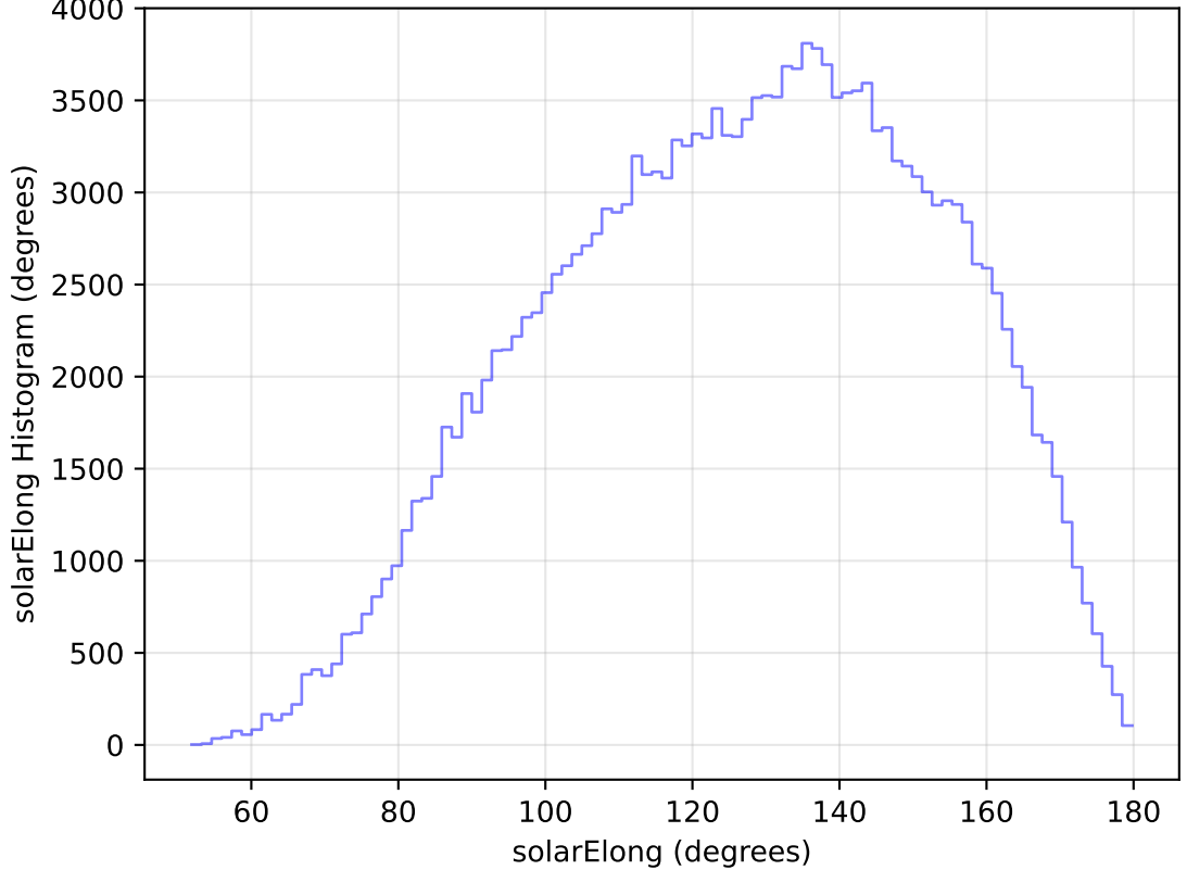
internal_u_expt45_nscale1.0v3.4_10yrs WFD g band: solarElong Histogram
