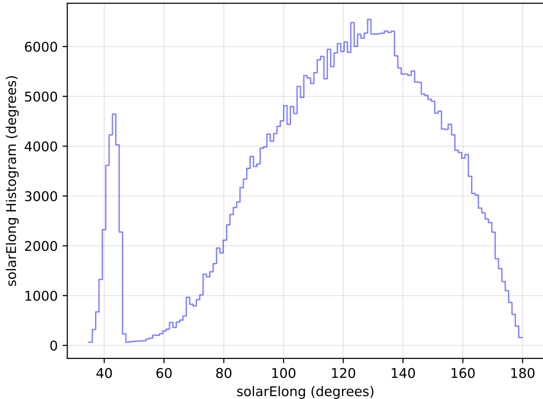
internal_u_expt45_nscale1.0v3.4_10yrs All sky z band: solarElong Histogram
