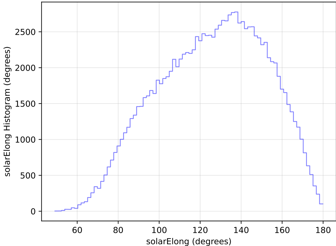
internal_u_expt45_nscale1.0v3.4_10yrs All sky u band: solarElong Histogram
