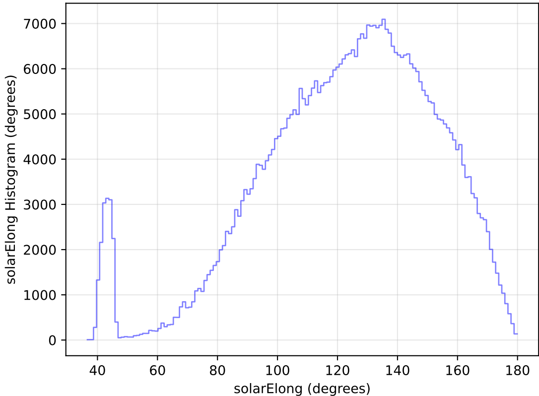
internal_u_expt45_nscale1.0v3.4_10yrs All sky r band: solarElong Histogram
