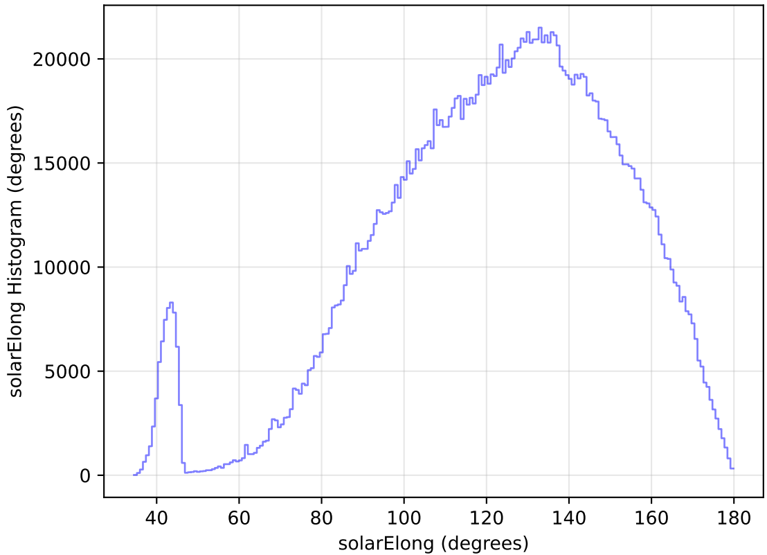
internal_u_expt45_nscale1.0v3.4_10yrs All sky all bands: solarElong Histogram
