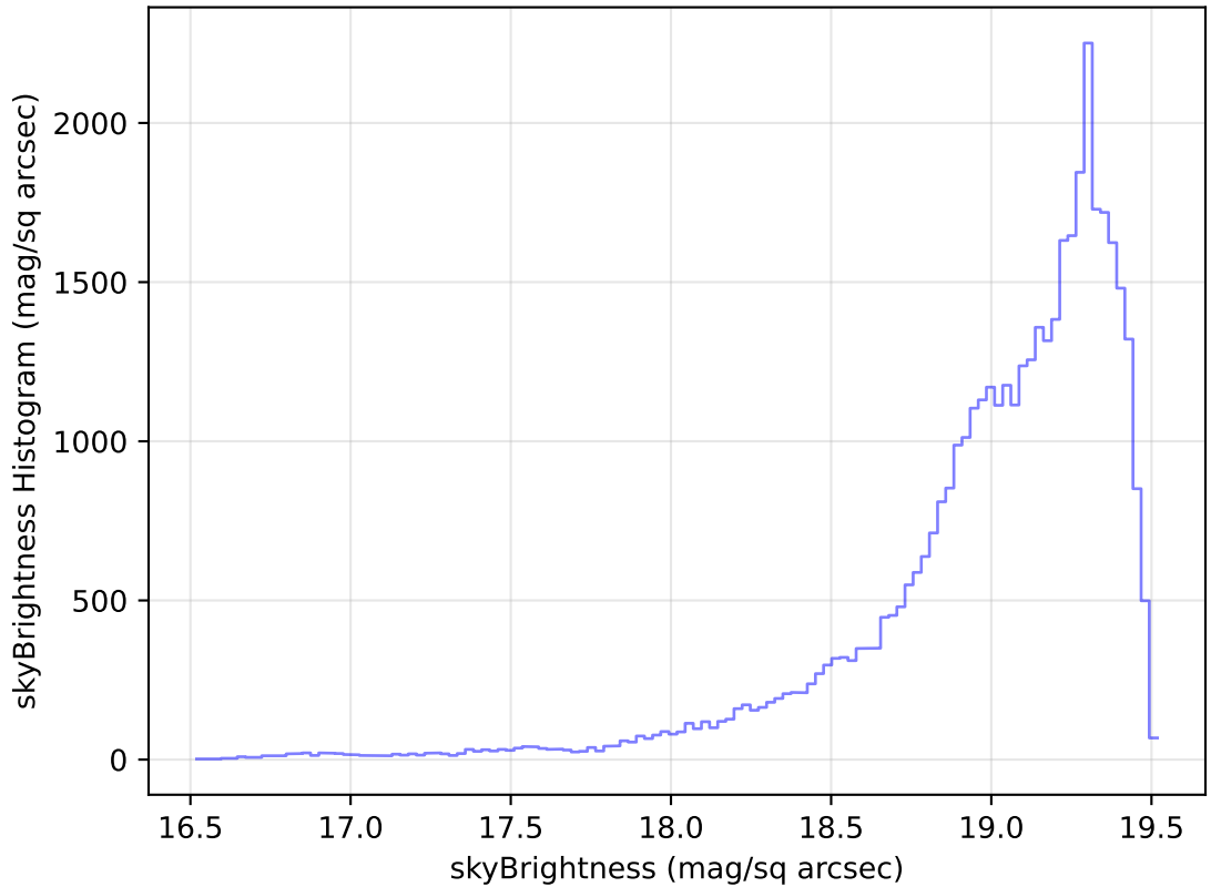
internal_u_expt45_nscale1.0v3.4_10yrs Yr 1 z band: skyBrightness Histogram
