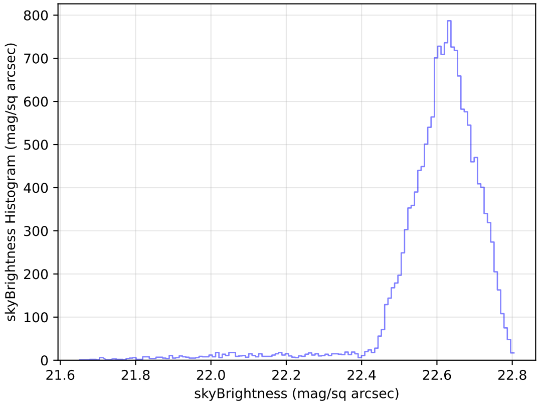
internal_u_expt45_nscale1.0v3.4_10yrs Yr 1 u band: skyBrightness Histogram
